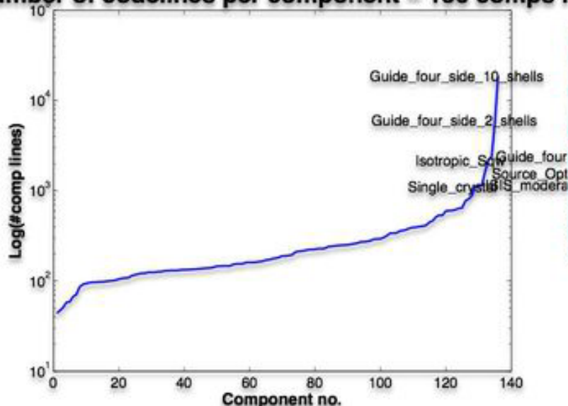
Number of codelines per component – 136 comps i
